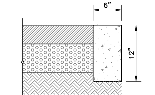
DETAIL A CONCRETE HEADER CURB
