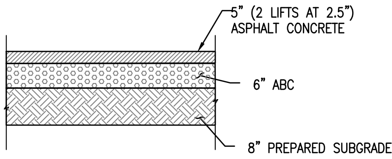
DETAIL B PAVEMENT SECTION:
