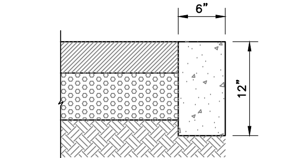
DETAIL A CONCRETE HEADER CURB
